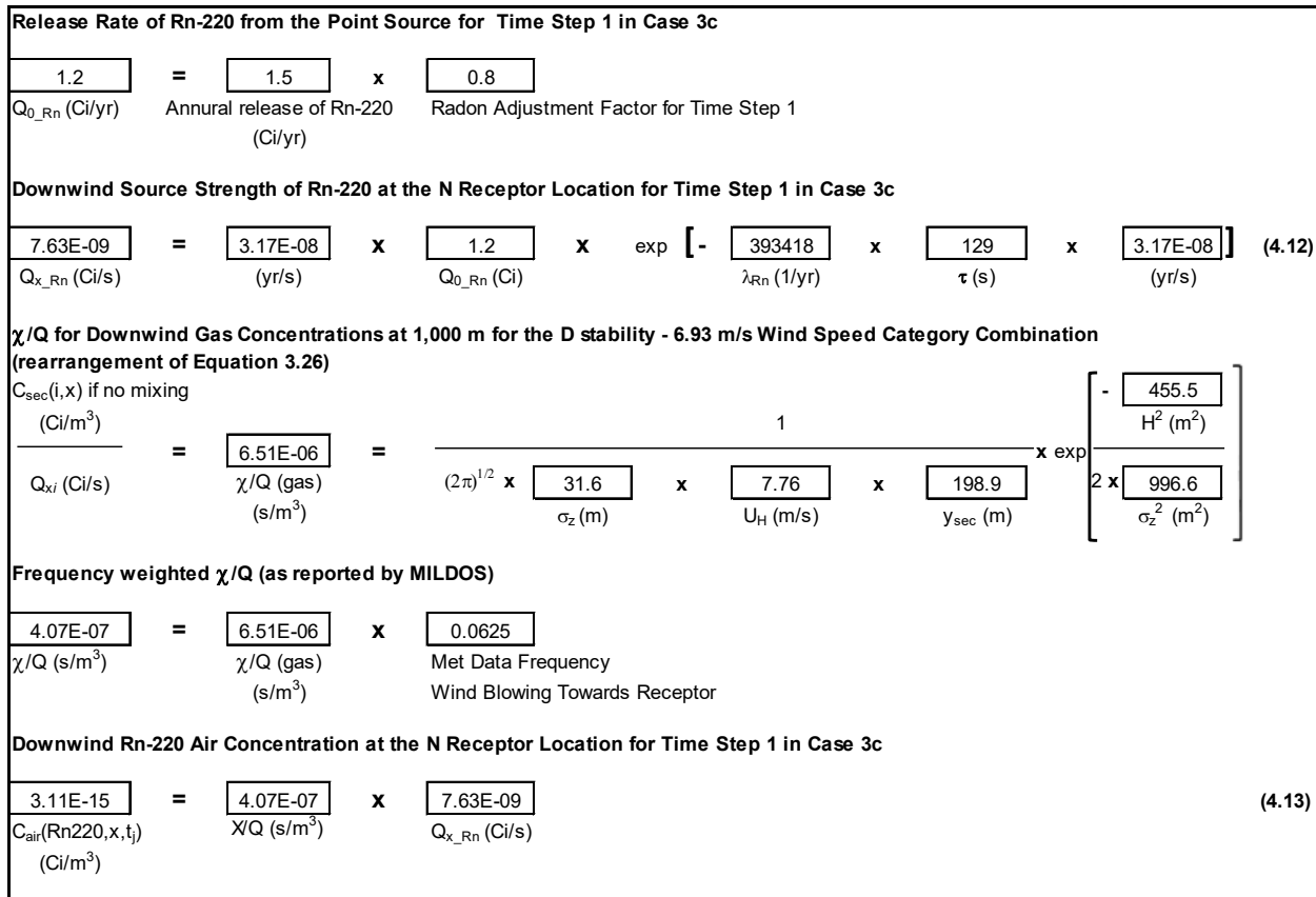
Figure 4-18 Hand Calculation of the Rn-220 Air Concentration at the N Receptor Location for Time Step 1 in Case 3c
