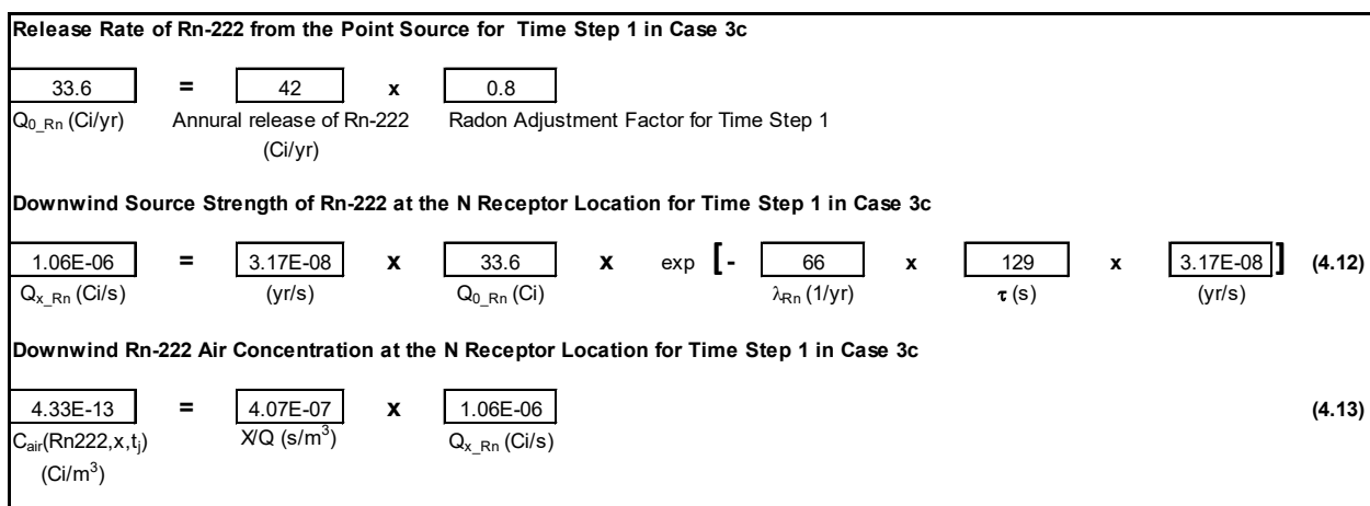
Figure 4-19 Hand Calculation of the Rn-222 Air Concentration at the N Receptor Location for Time Step 1 in Case 3c
