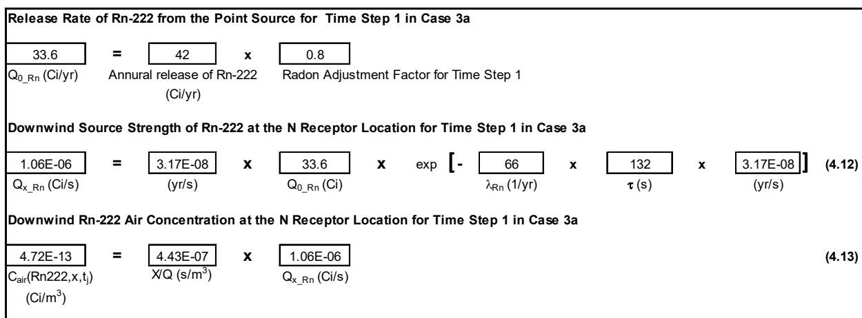
Figure 4-13 Hand Calculation of the Rn-222 Air Concentration at the N Receptor Location for Time Step 1 in Case 3a
