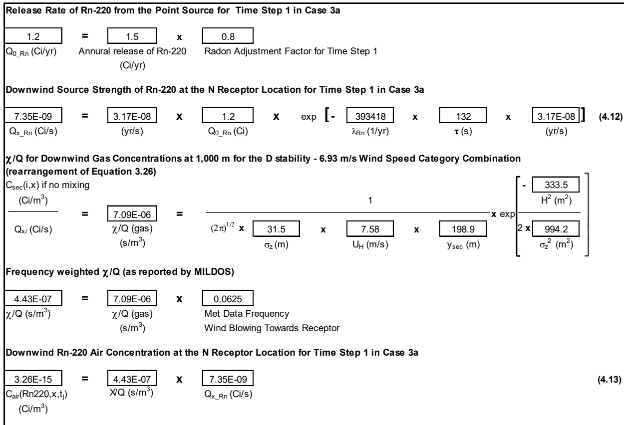
Figure 4-12 Hand Calculation of the Rn-220 Air Concentration at the N Receptor Location for Time Step 1 in Case 3a
