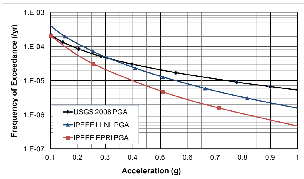
Figure 2 Comparison of PGA exceedance frequencies at the reference plant
