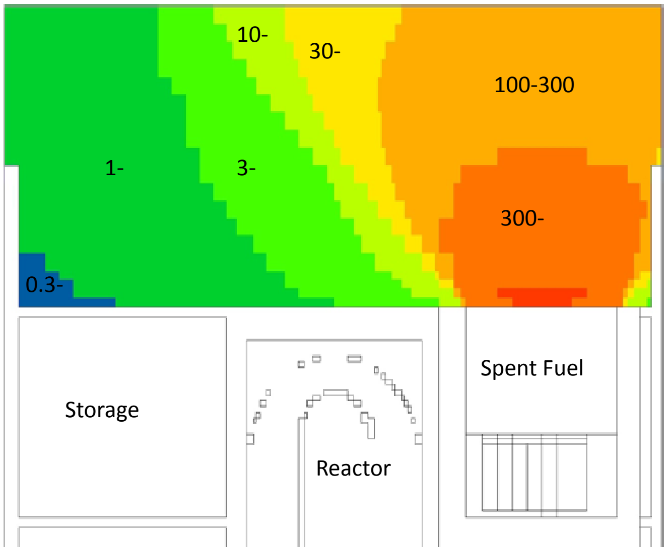
Figure 36 Approximate dose rate of elevation contours, water at top of fuel hardware, around the time of defueling (rem per hour).
