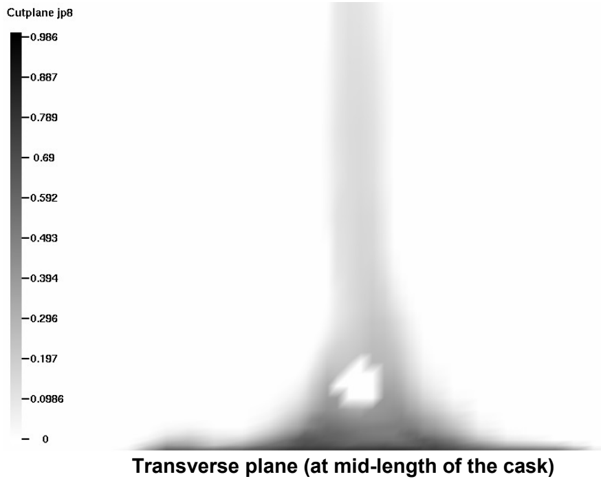
Figure 4-39 Fuel concentration plots CAFE fire analysis of the Truck-DU cask lying on ground
