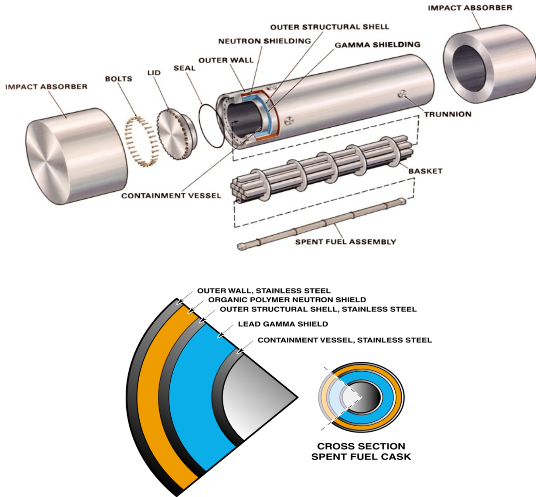
Figure 2-1 The upper figure is an exploded view of a generic spent fuel cask Figure source: (Sandia National Laboratories archive) The lower figure is a cross-section of the layers of the cask wall.
