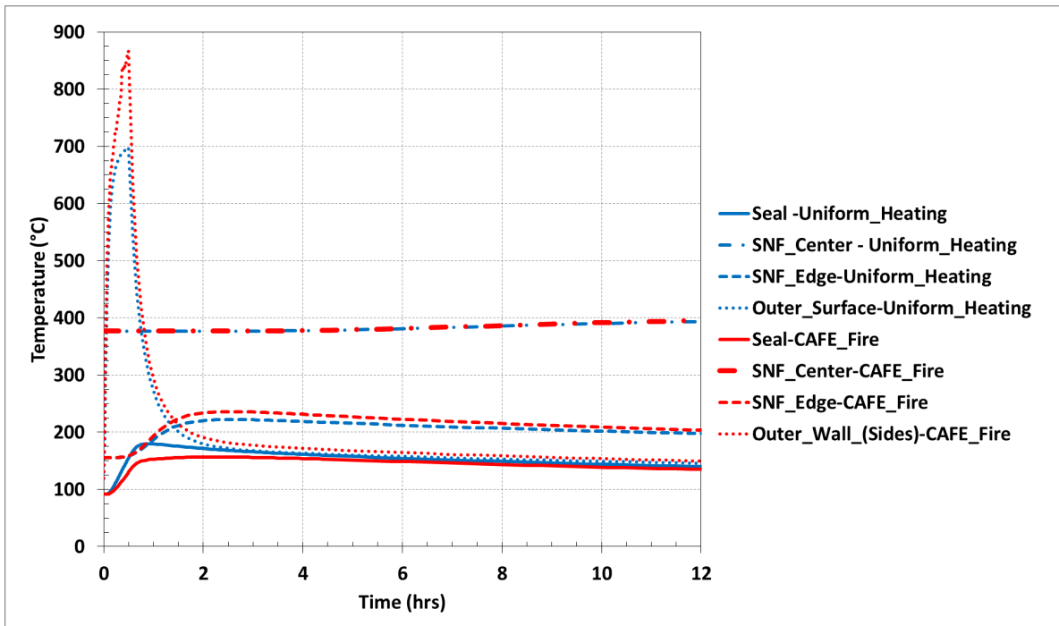
Figure 4-11 Comparison of regulatory fire analysis for Rail-Steel cask: Uniform heating vs. CAFE fire
