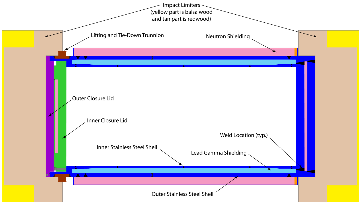
Figure 1-2 Photograph and cross-section of the NAC-STC cask Figure source: (courtesy of NAC International)
