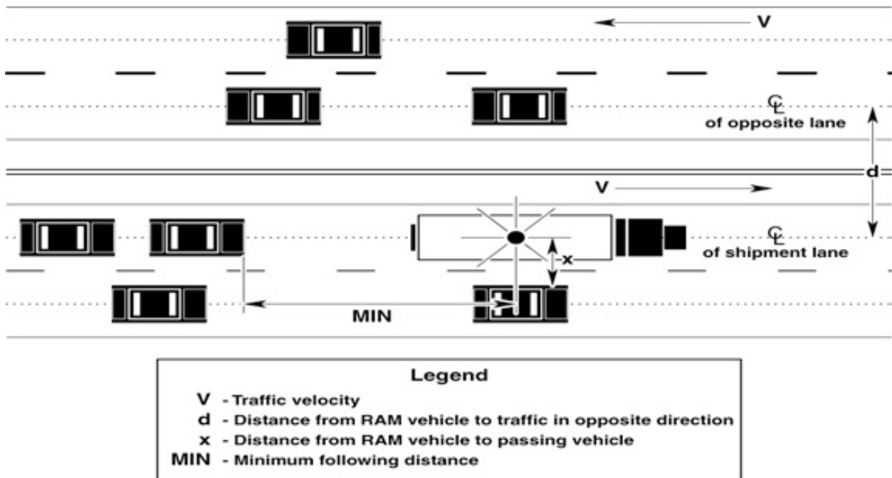
Figure B-14 Parameters for calculating doses to occupants of highway vehicles sharing the route with the radioactive shipment (from Figure 3-2 of Neuhauser et al., 2000)
