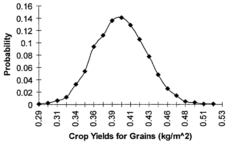
Figure 6.32 PDF for crop yields for grain
