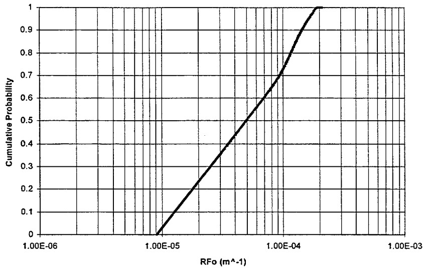
Figure 5.7 Cumulative probability function for RF.
