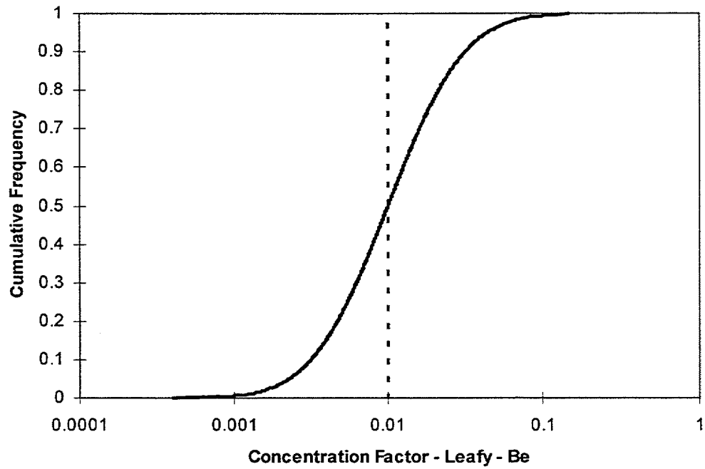
Figure 6.85 Cumulative frequency of sampled B 10v for Be in leafy vegetables (dashed vertical line = NUREG/CR-5512, Vol. 1, default)
