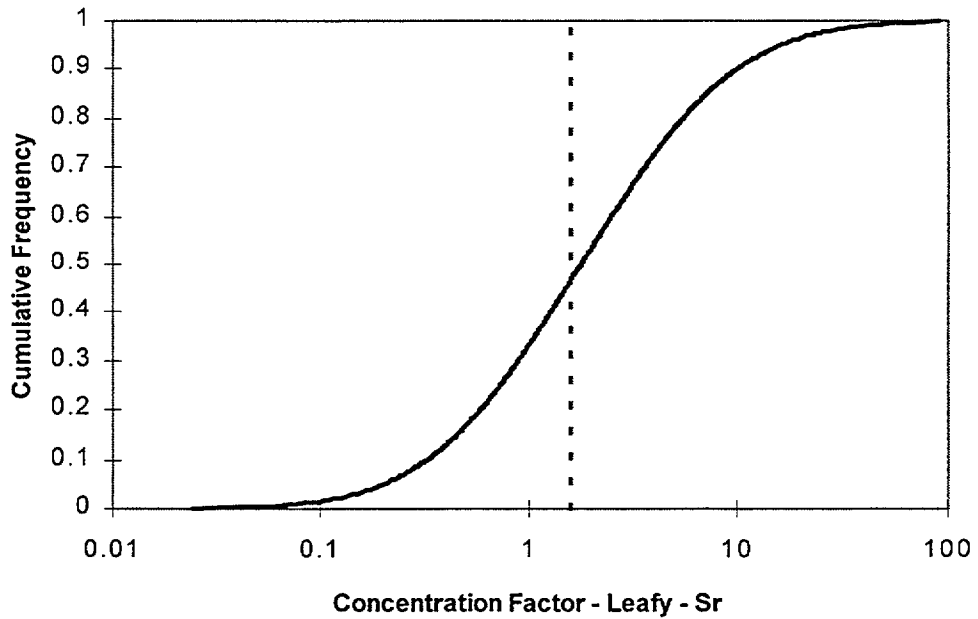
Figure 6.86 Cumulative frequency of sampled B 10v for Sr in leafy vegetables (dashed vertical line = NUREG/CR-5512, Vol. 1, default)
