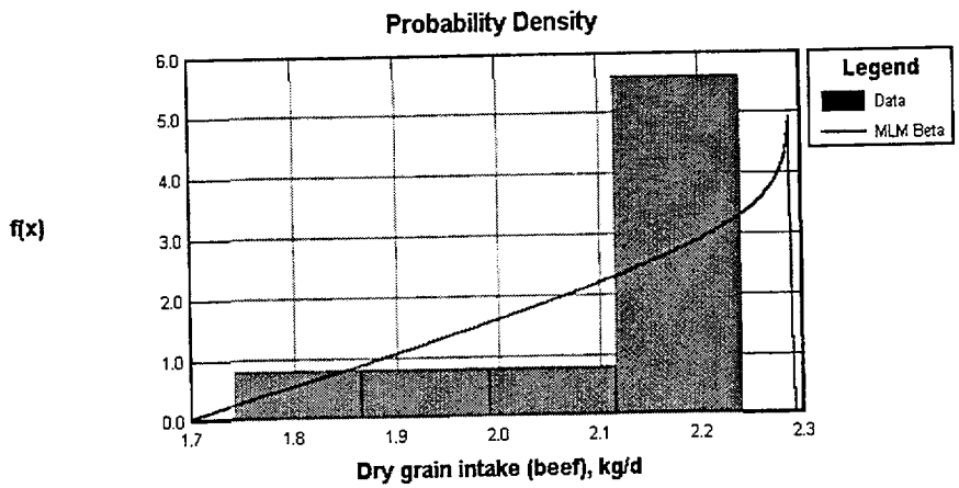
Figure 6.41 Calculated probability distribution for stored grain consumed by beef cattle
