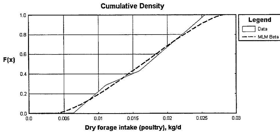
Figure 6.54 Cumulative distribution for forage consumed by poultry
