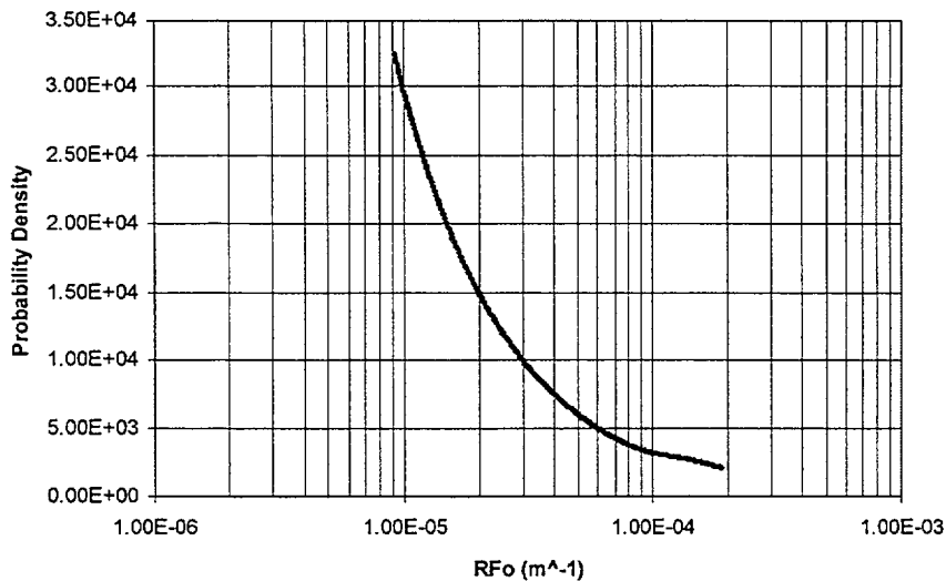
Figure 5.8 Proposed probability density function for RF.
